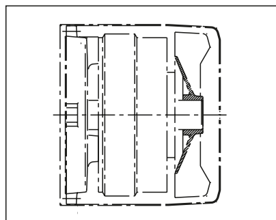
Special version Type of cooling IC 411, self-ventilated with built-on brake
