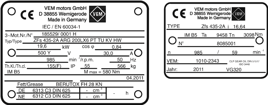
Figure 8: Example of a name plate for geared roller table motors
